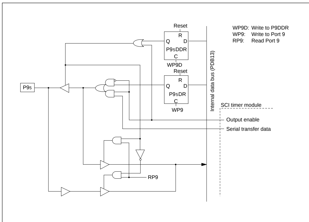
Figure C-9 (c) Schematic Diagram of Port 9, Pin P95
