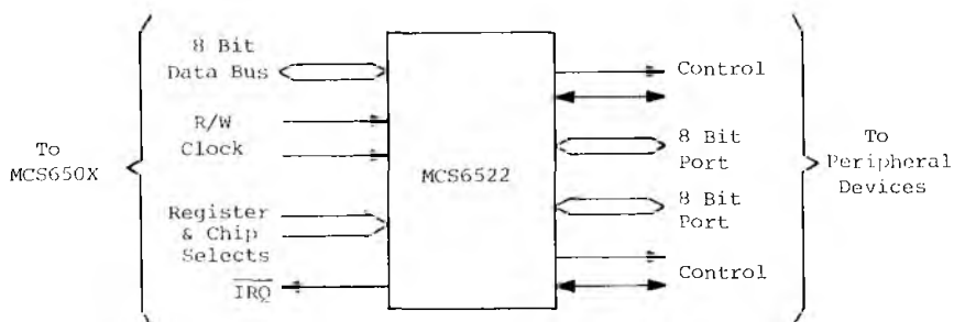
MCS6522 Interface Diagram
