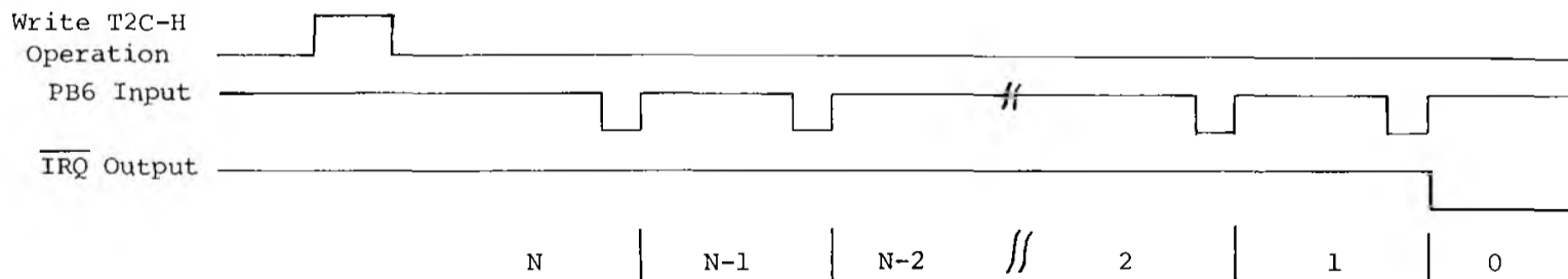
Figure 7. Timer 2 Pulse Counting Mode
