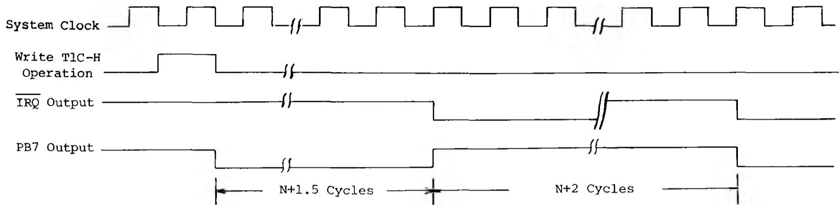
Figure 6. Timer 1 "Free-Running" Mode
